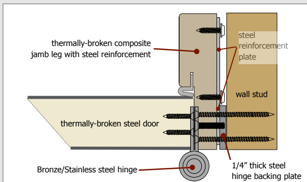
Standard Steel Reinforced Jamb Legs Section drawing of the thermally broken jamb legs
